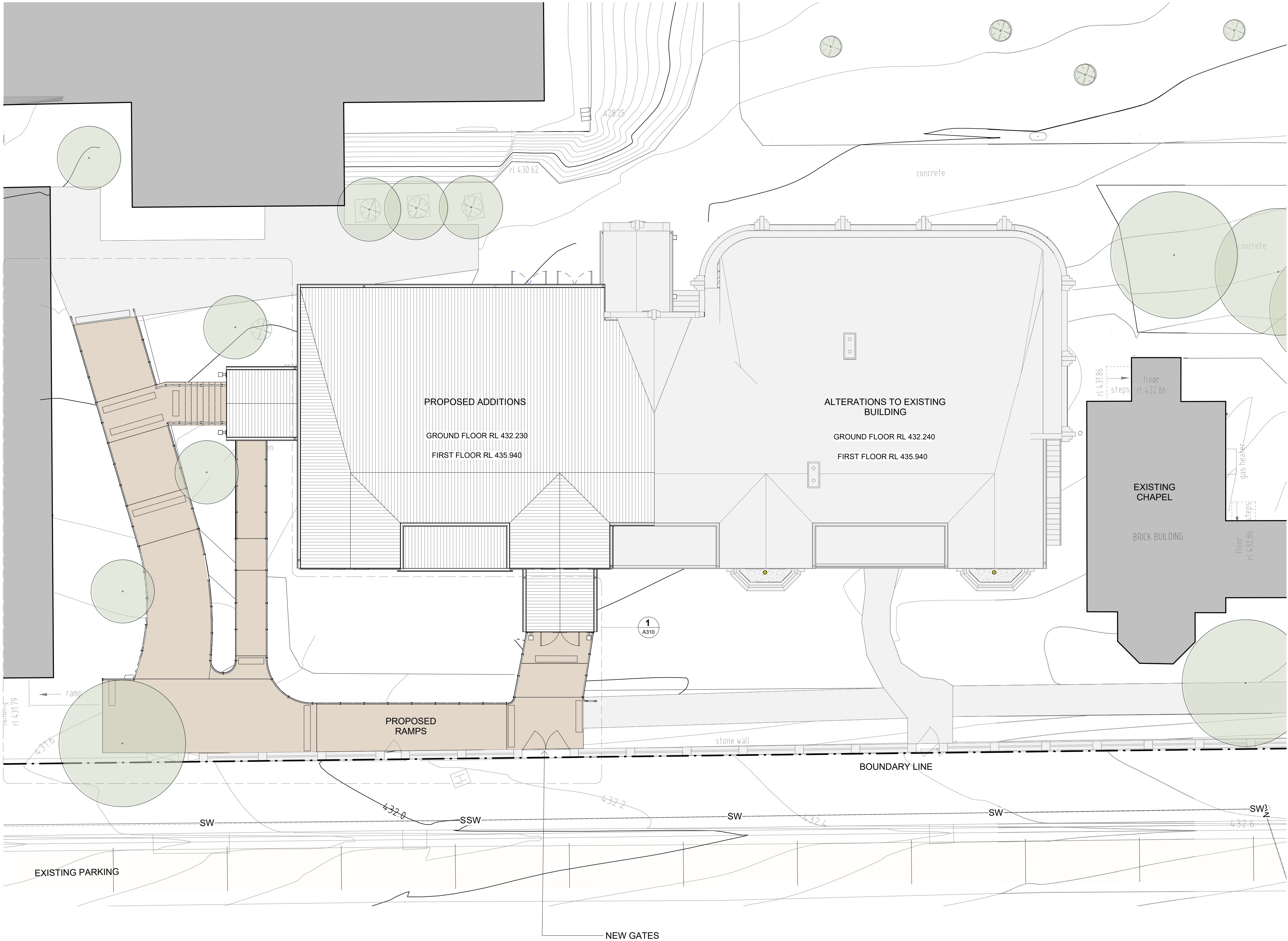
1 SITE - PROPOSED PLAN A205 1:100
